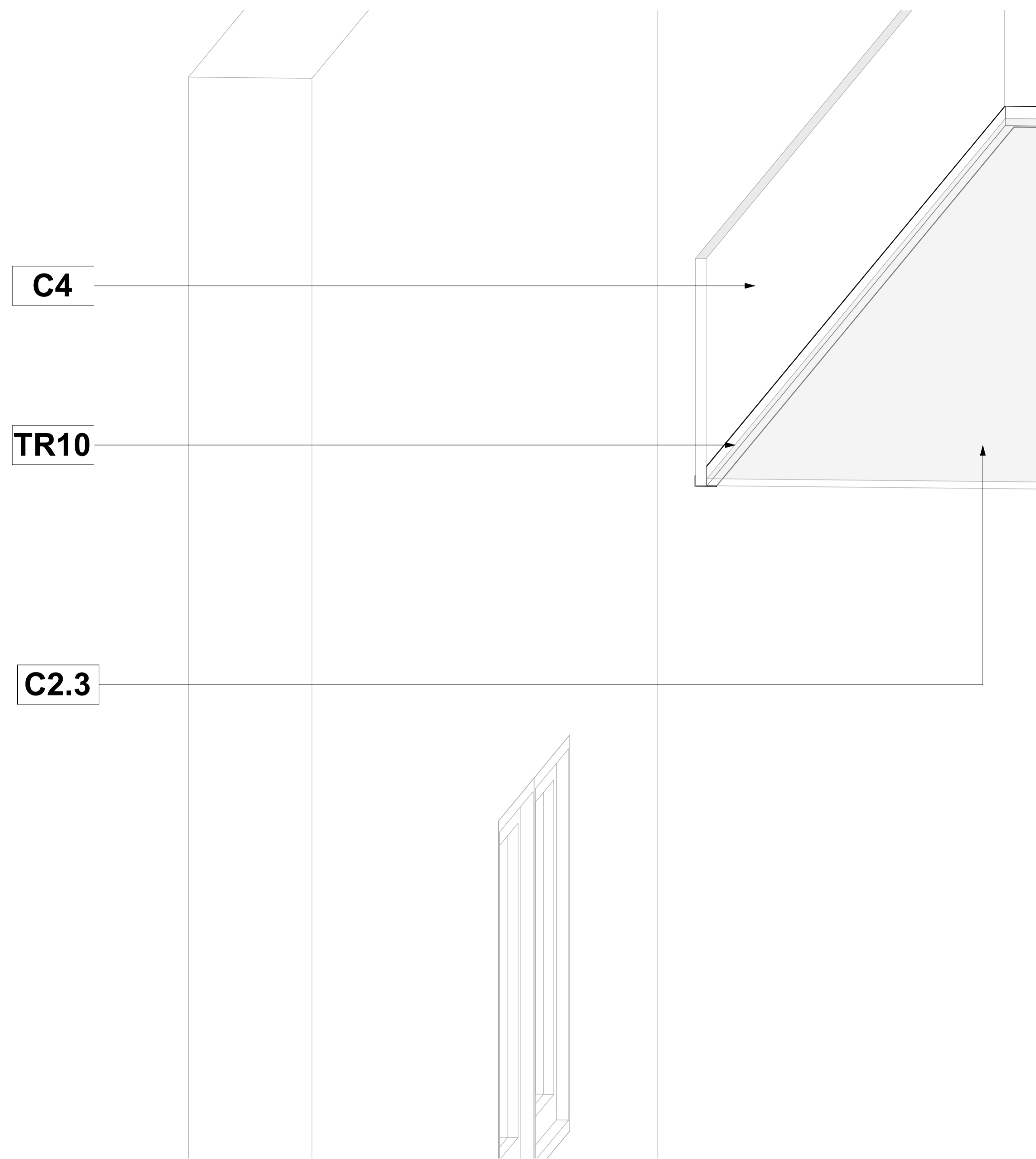
TR10 - Fascia Trim - 3D
