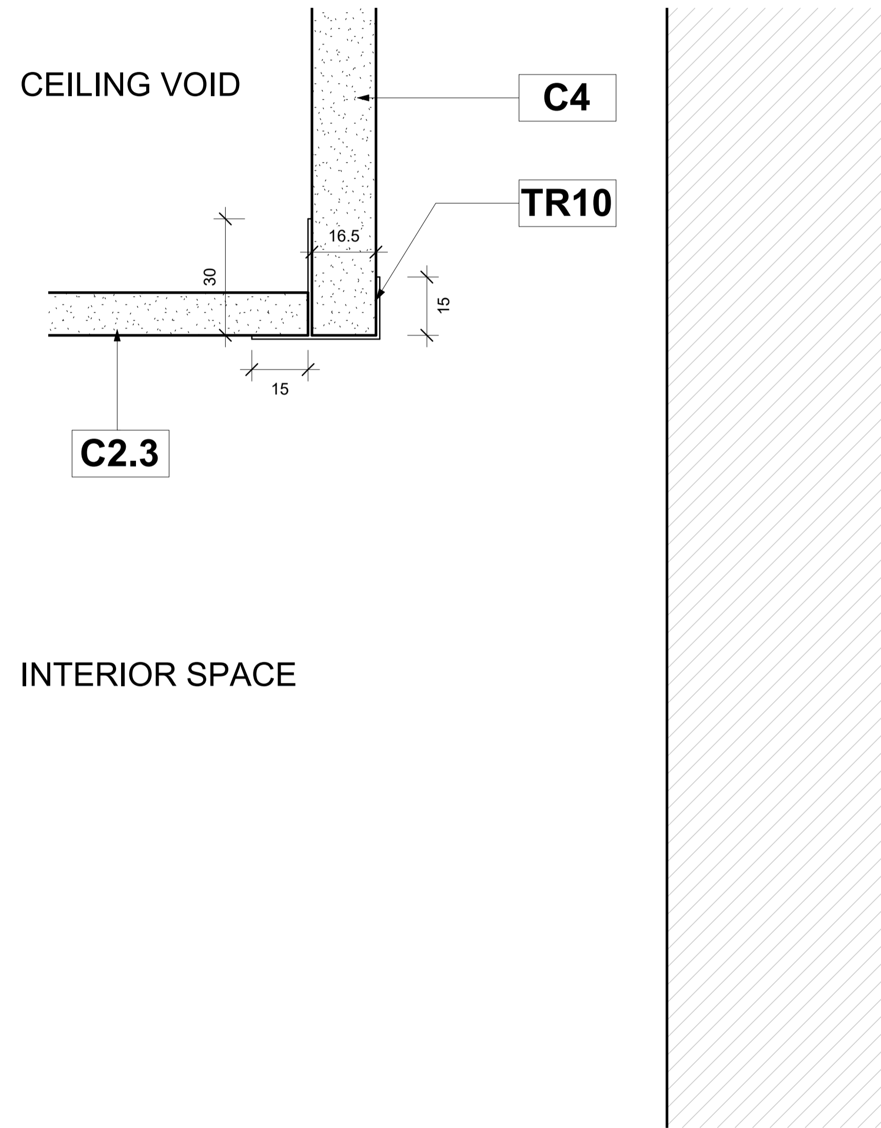
TR10 - Fascia Trim - Section
