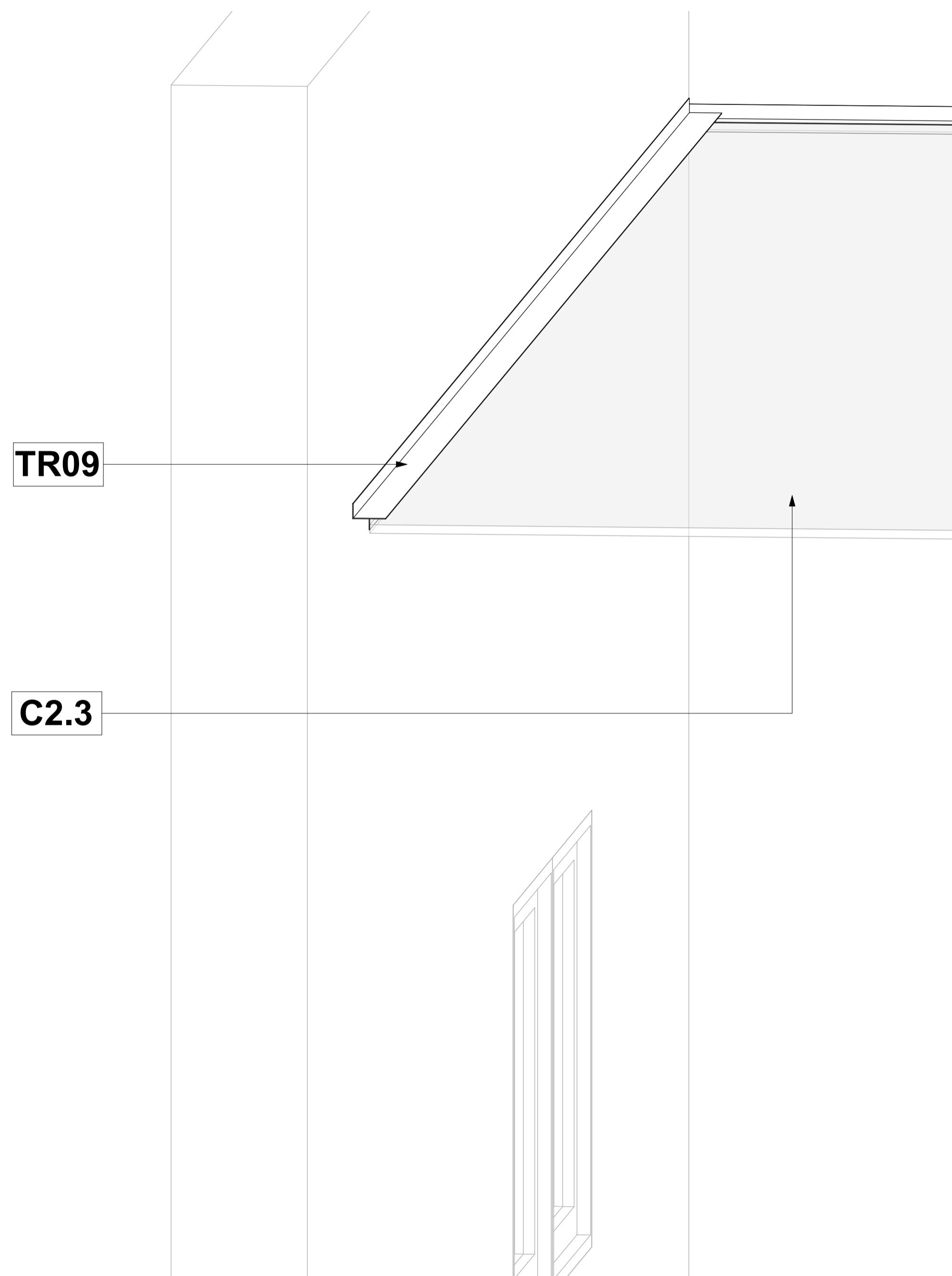
TR09 - 15mm Steel Plaster Trim for 12mm JUMBO Board - 3D
