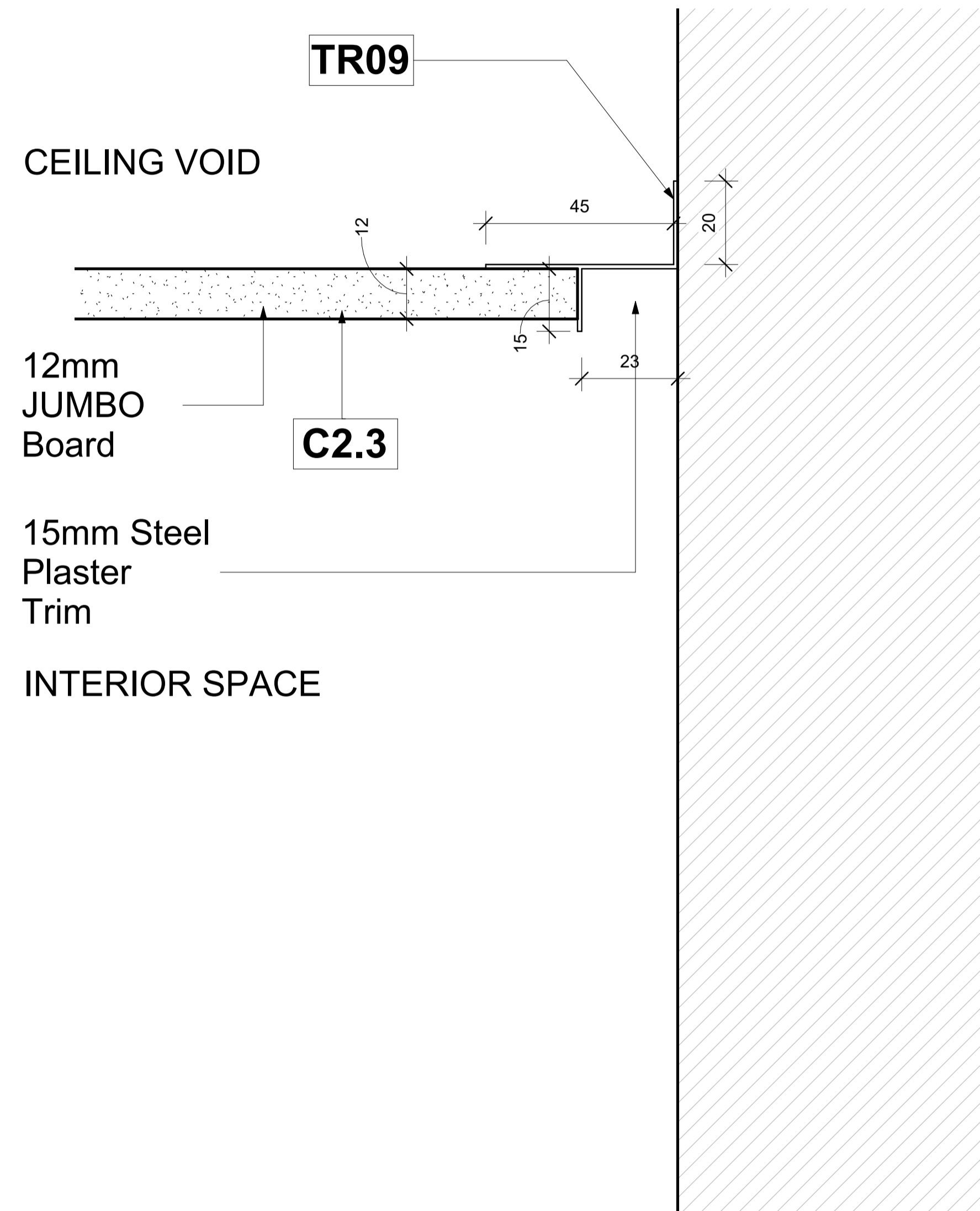
TR09 - 15mm Steel Plaster Trim for 12mm JUMBO Board - Section
