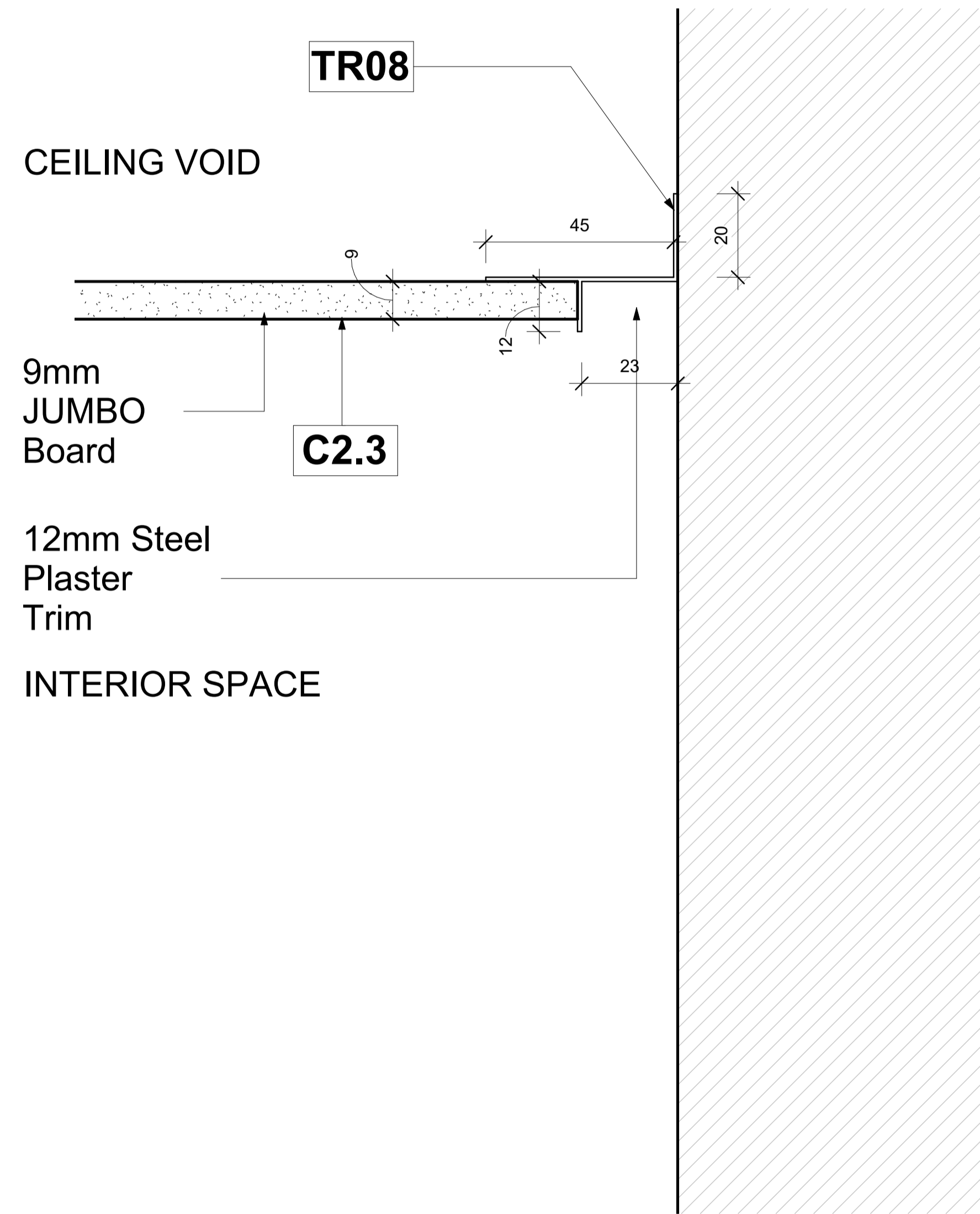
TR08 - 12mm Steel Plaster Trim for 9mm JUMBO Board - Section
