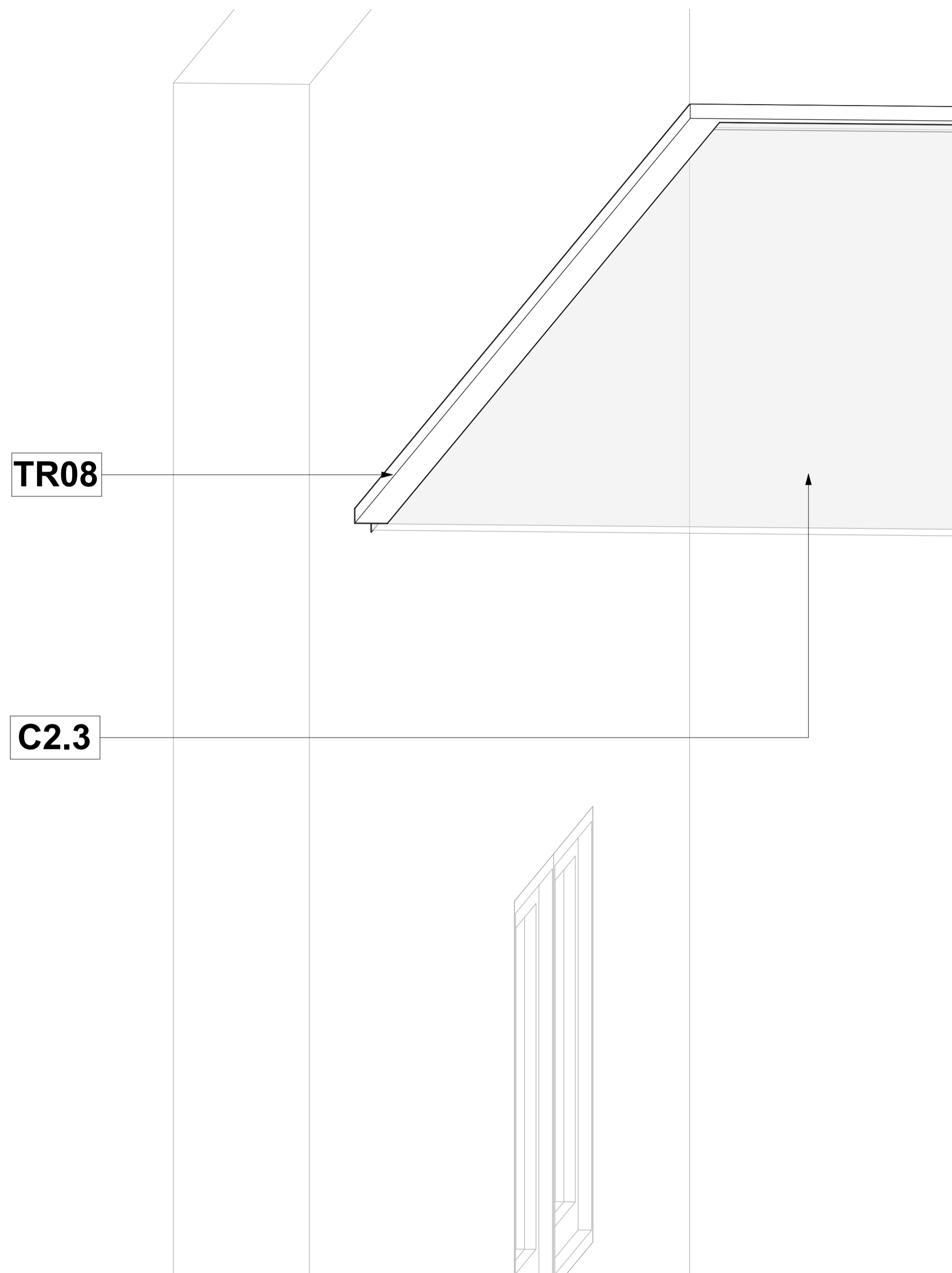
TR08 - 12mm Steel Plaster Trim for 9mm JUMBO Board - 3D
