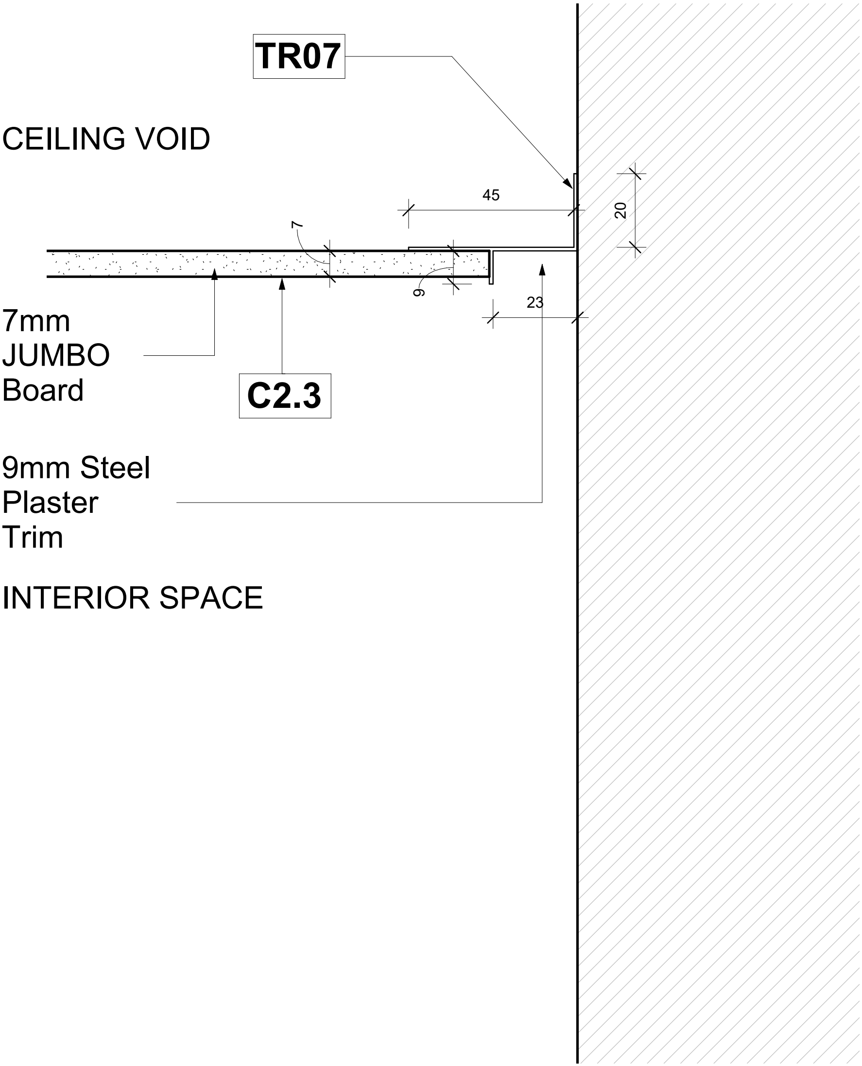
TR07 - 9mm Steel Plaster Trim for 7mm JUMBO Board - Section
