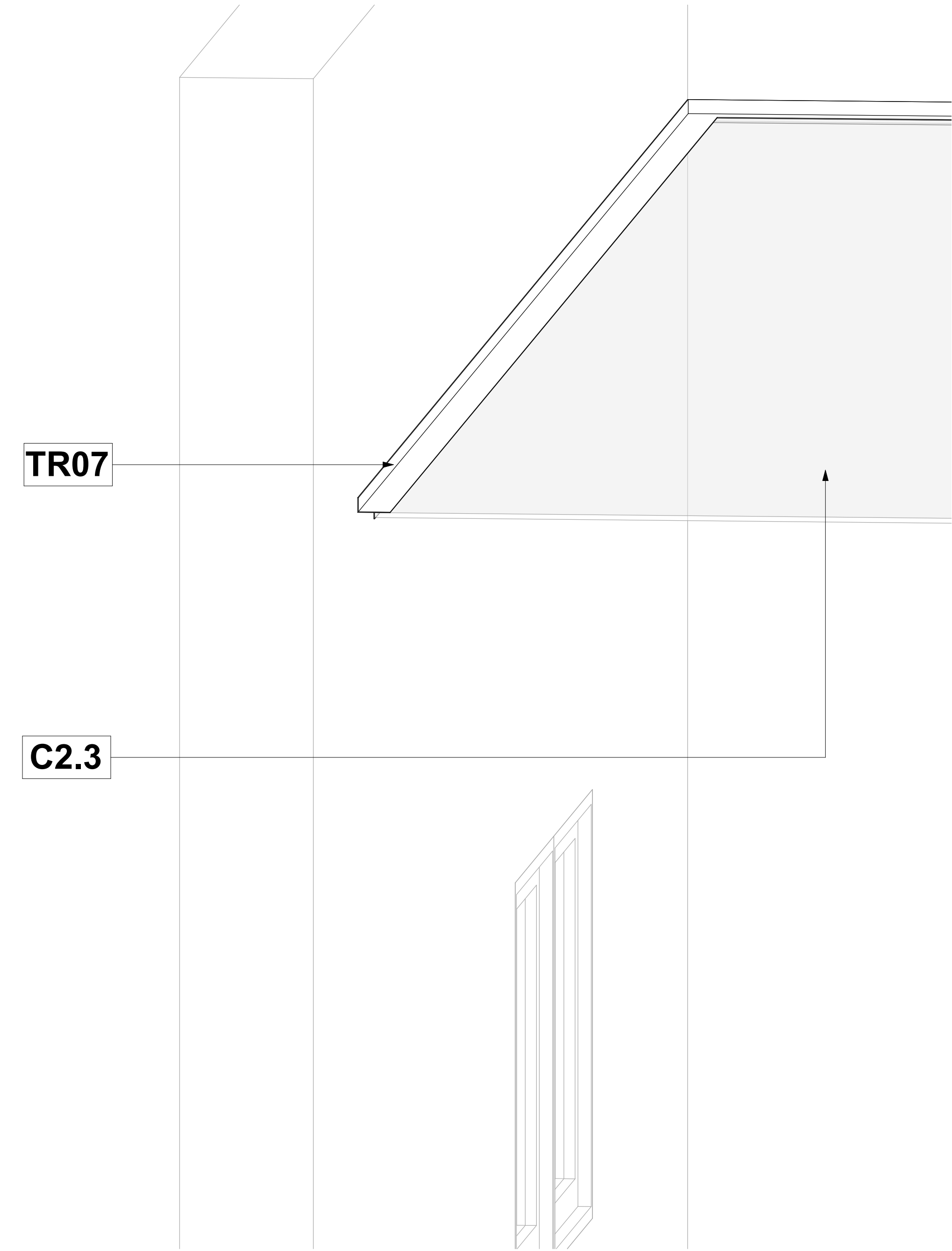
TR07 - 9mm Steel Plaster Trim for 7mm JUMBO Board - 3D
