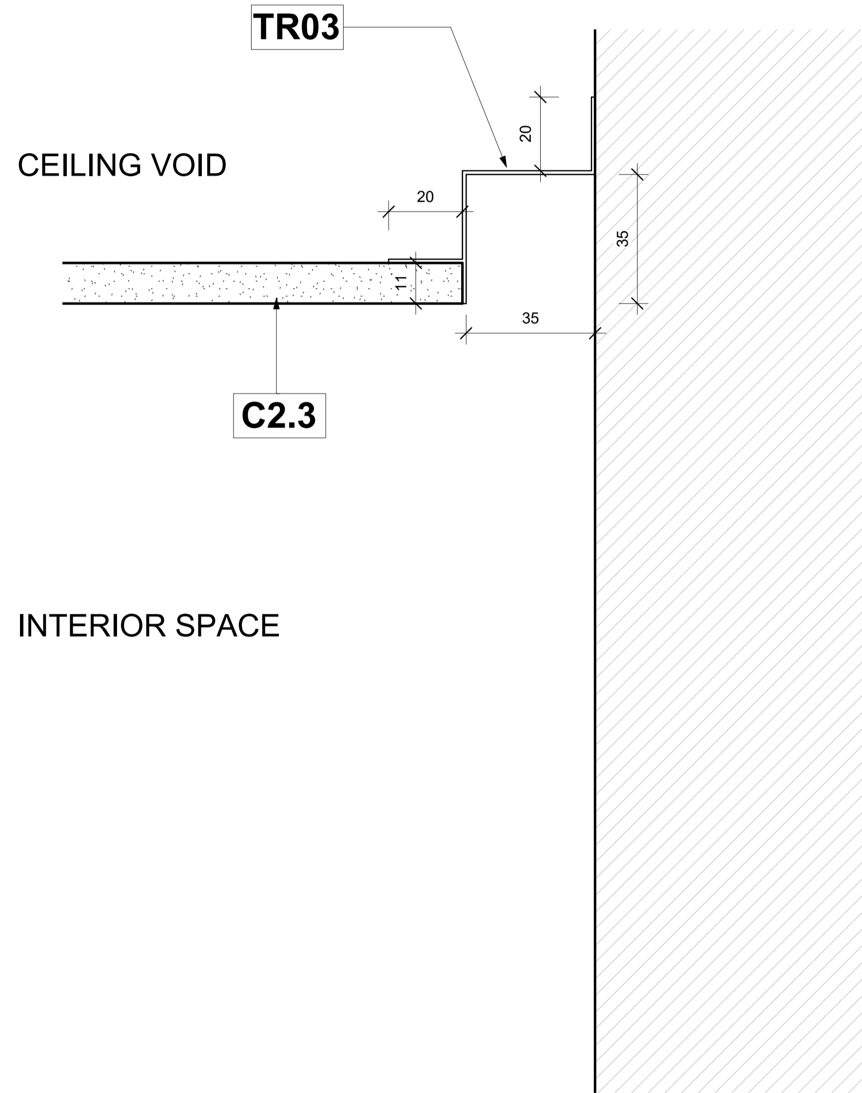
TR03 - PS35 Plaster Trim 35 x 35 - Section
