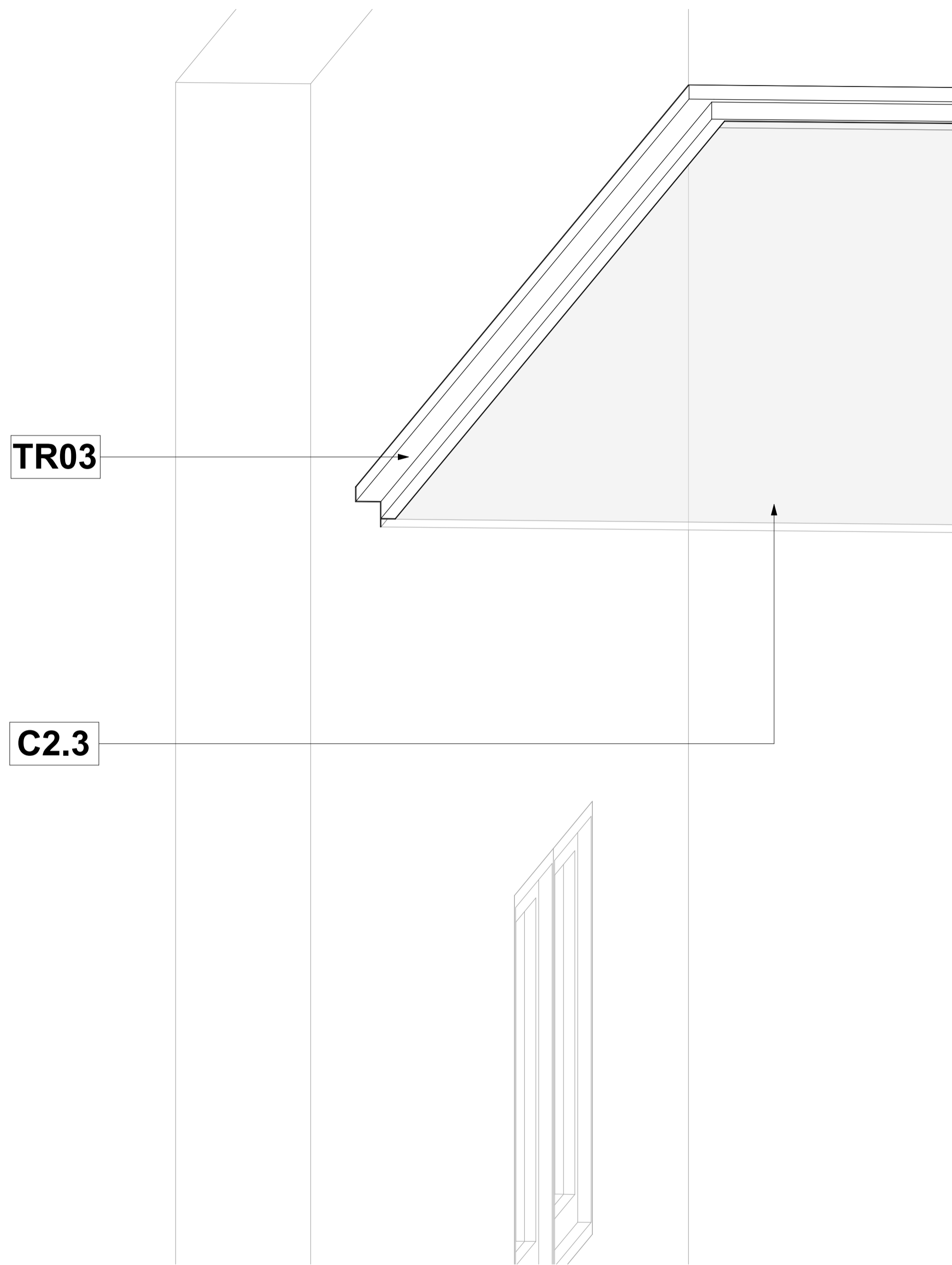
TR03 - PS35 Plaster Trim 35 x 35 - 3D
