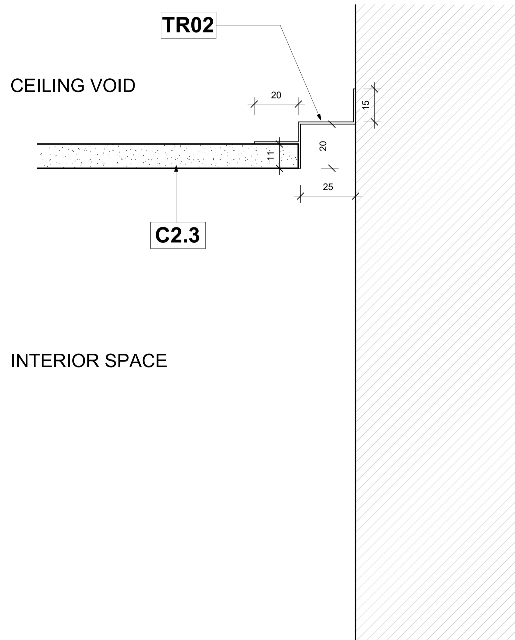
TR02 - PS2 Plaster Trim 25 x 20 - Section
