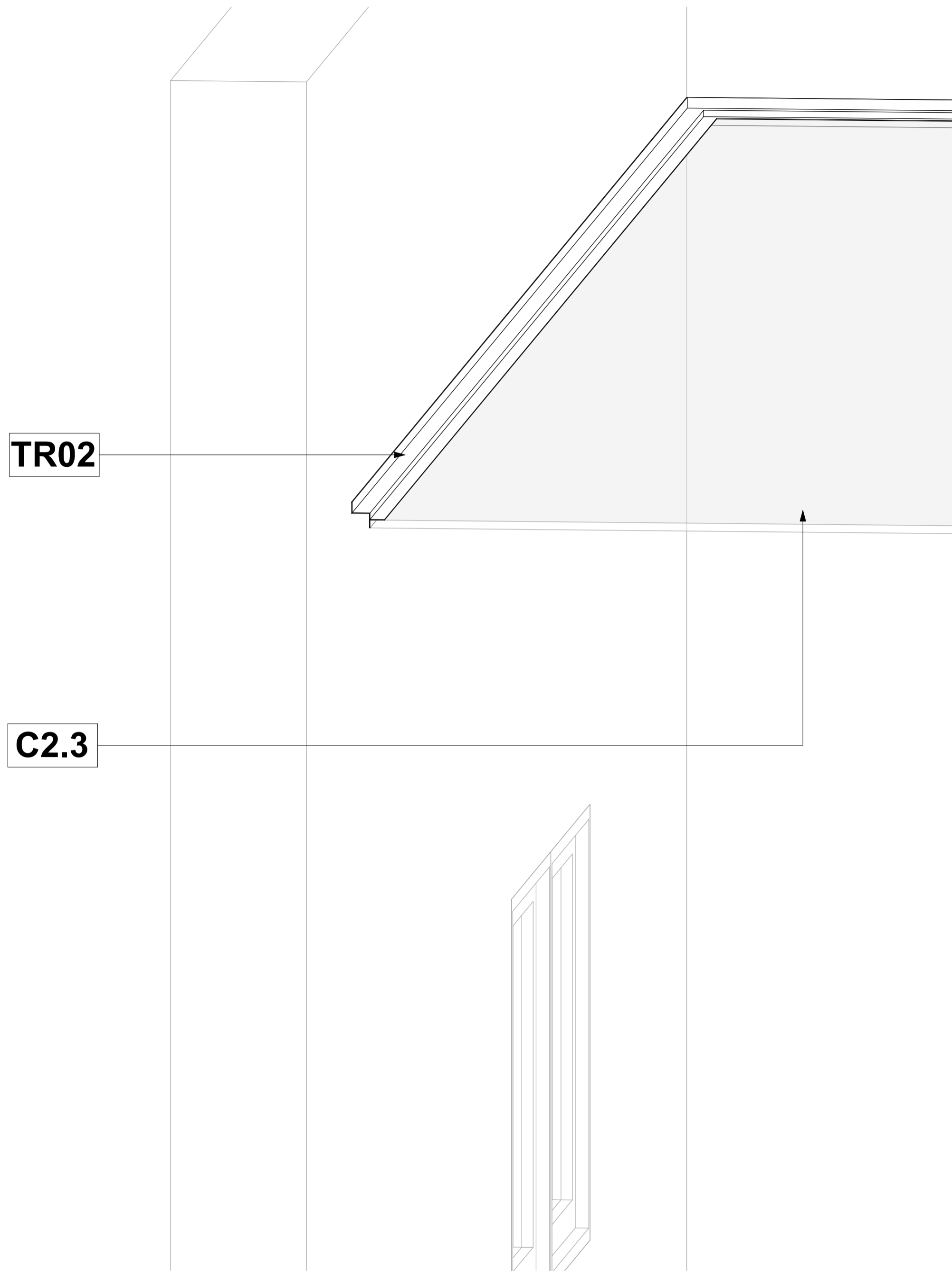
TR02 - PS2 Plaster Trim 25 x 20 - 3D
